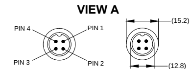
4 PIN MALE MATING FACE
